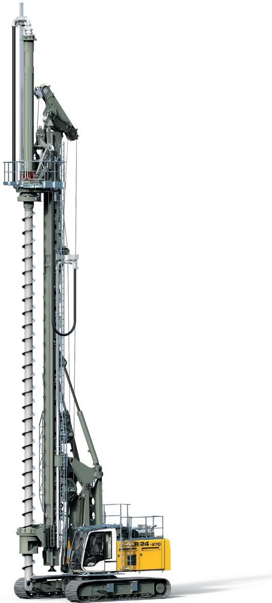
Auger with auger cleaner
